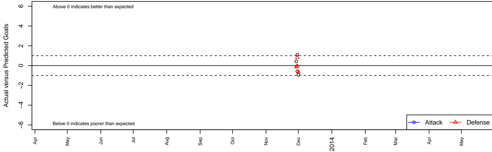
Futeca Camp Elite B95 Dots are actual minus expected GF (blue circles) and GA (red triangles). Blue line is smoothed change in attack strength. Red is smoothed change in defense strength.
